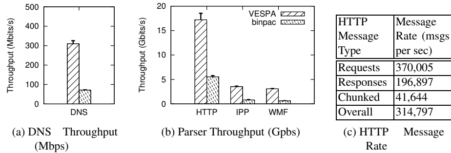
Fig. 3: Vulnerability Signature Matcher Performance
